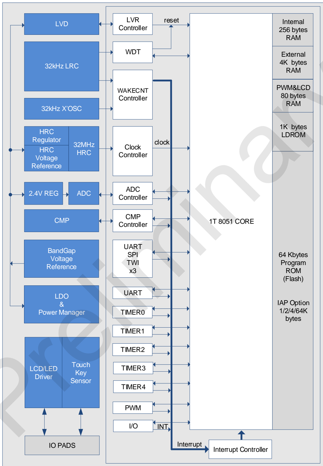
SC8FT67 BLOCK DIAGRAM
