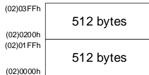
SC8FT67 1 Kbytes LDROM Sector 示意
