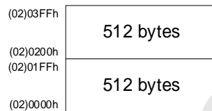
SC95F852X 1 Kbytes LDROM Sector 示意
