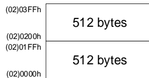
SC95F852X 1 Kbytes LDR0M Sector 示意
