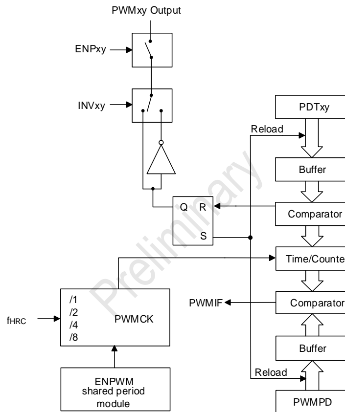
SC95F861X PWM Independent mode block diagram
