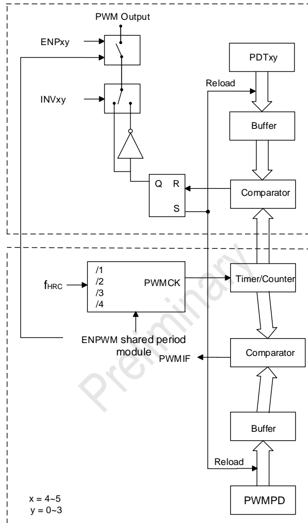
SC95F861X PWM Structure diagram
