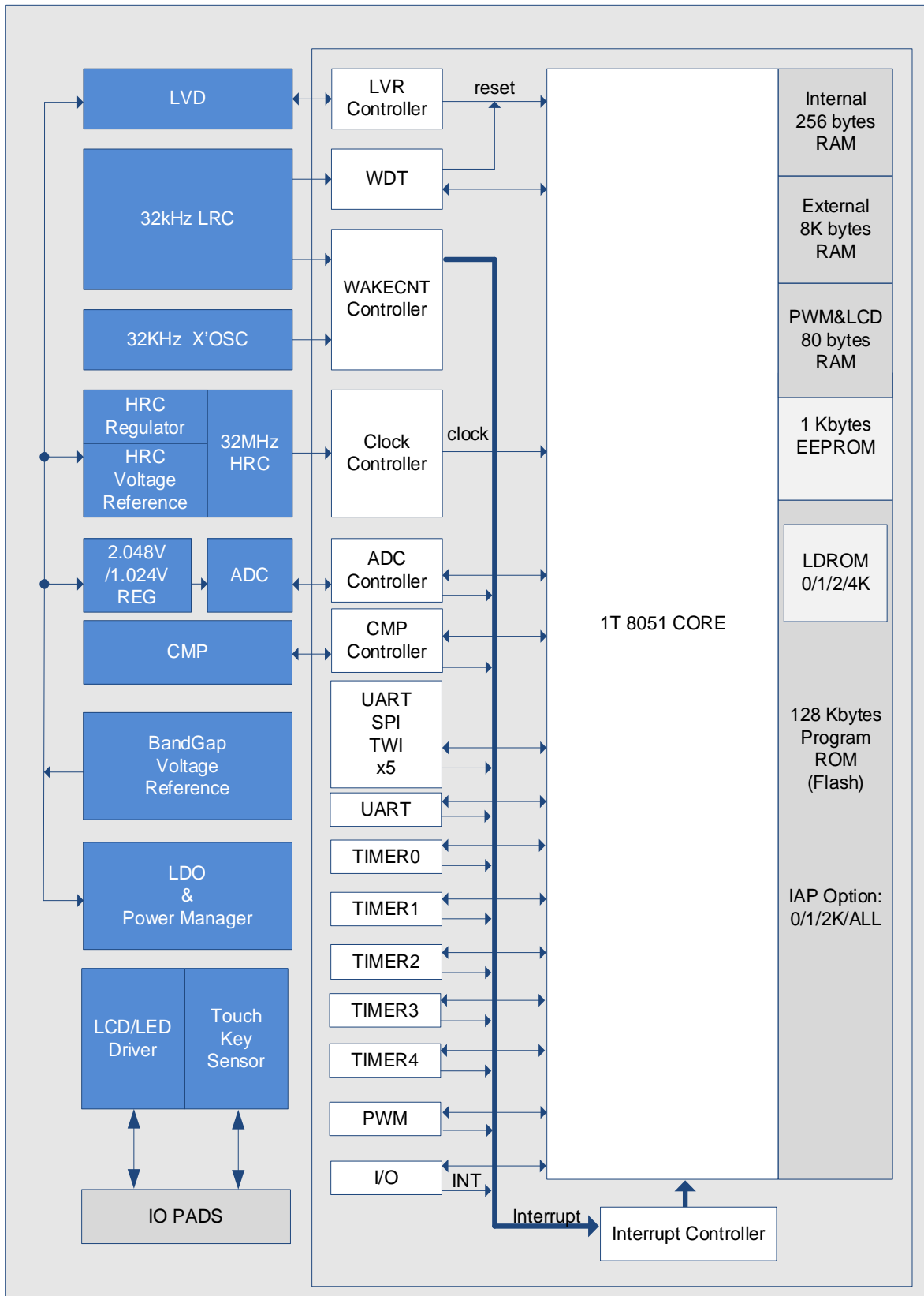
SC95F873X BLOCK DIAGRAM
